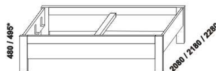
990 / 1084 / 1284 1484 / 1684 / 1884 / 2084 postel MILET NR-NR 90, 100, 120 x 200, 210, 220 140, 160, 180, 200 x 200, 210, 220
