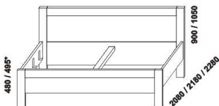
990 / 1084 / 1284 1484 / 1684 / 1884 / 2084 postel MILET, čelo 1 – plné 90, 100, 120 x 200, 210, 220 140, 160, 180, 200 x 200, 210, 220
