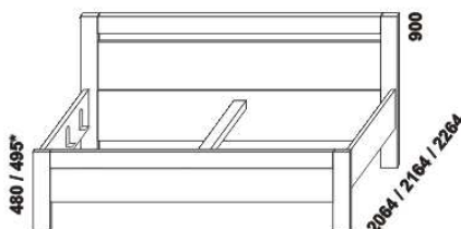
990 / 1284 / 1484 / 1684 / 1884 postel LINE, čelo 2 - s otvorem 90, 120, 140, 160, 180 x 200, 210, 220
