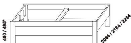
990 / 1284 / 1484 / 1684 / 1884 postel LINE NR-NR 90, 120, 140, 160, 180 x 200, 210, 220
