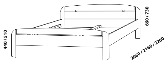
960 / 1060 / 1260 / 1460 / 1660 / 1860 / 2060 postel NIKOLA 90, 100, 120 × 200, 210, 220 140, 160, 180, 200 × 200, 210, 220
